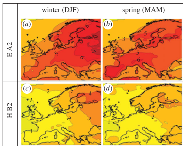
Figure 5. Projected change in air temperature for Europe: 2070–2100. The mean difference between scenario (2071–2100) and control (1961–1990) outputs for air temperature ( ^{\circ}\text{C} ) across Europe in winter (DJF) and spring (MAM) for the ECHAM4/OPYC3-RCAO A2 (E A2) (a and b) and HadAM3H-RCAO B2 (H B2) (c and d) scenarios.
